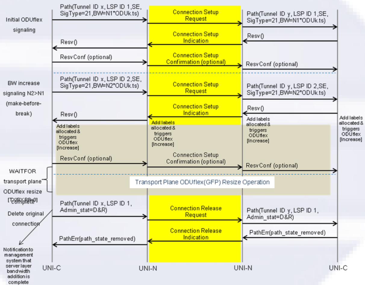
Figure 19: ODUflex Hitless Bandwidth Increase
