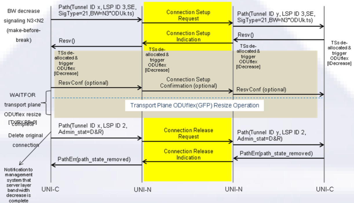
Figure 20: ODUflex Hitless Bandwidth Decrease
