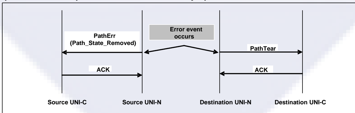
Figure 14 - Forced Connection Tear-Down by the Network
