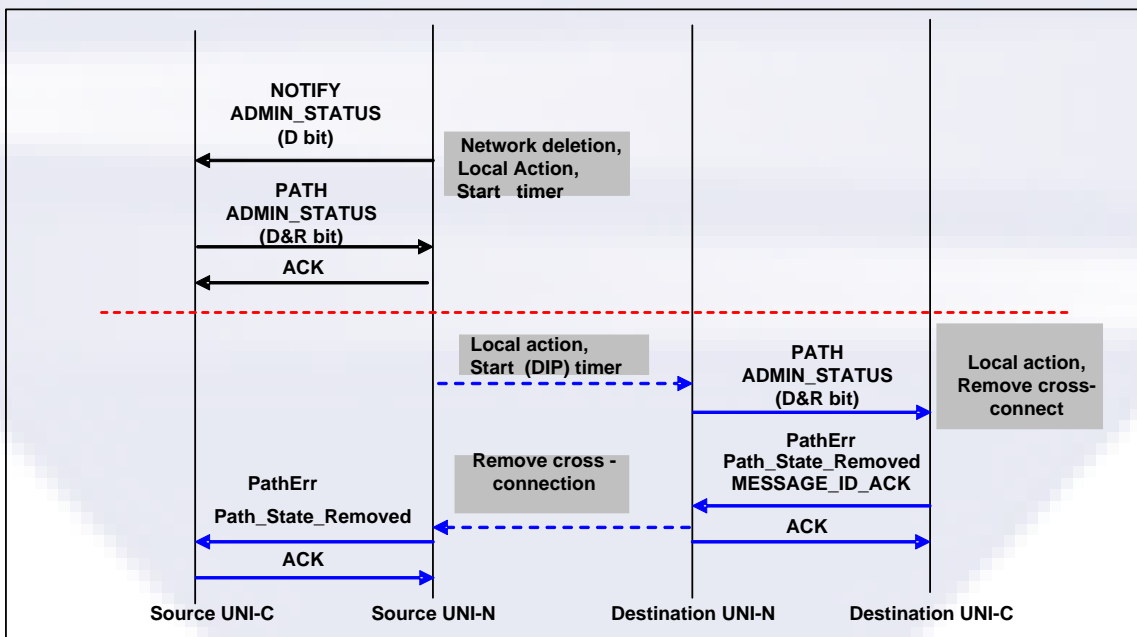
Figure 12 - Connection Teardown Initiated by the Source UNI-N
